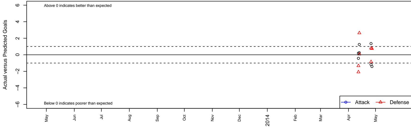
Wenatchee Fire Black G02 Dots are actual minus expected GF (blue circles) and GA (red triangles). Blue line is smoothed change in attack strength. Red is smoothed change in defense strength.
